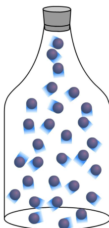
The particles in a gas
